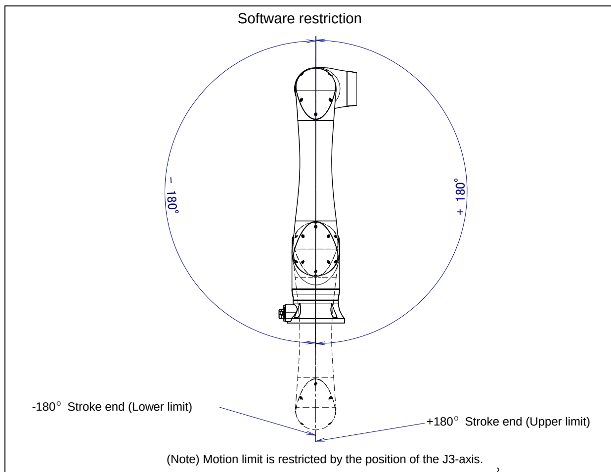
Fig. 3.3 (c) J2-axis motion limit (CRX-10iA, CRX-10iA/L)
