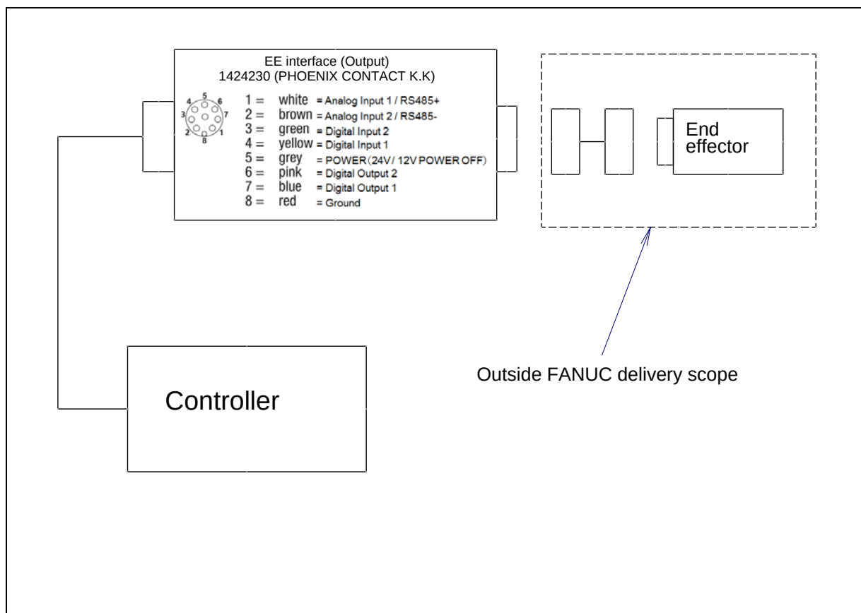
Fig. 5.1 (c) Pin layout for EE interface
