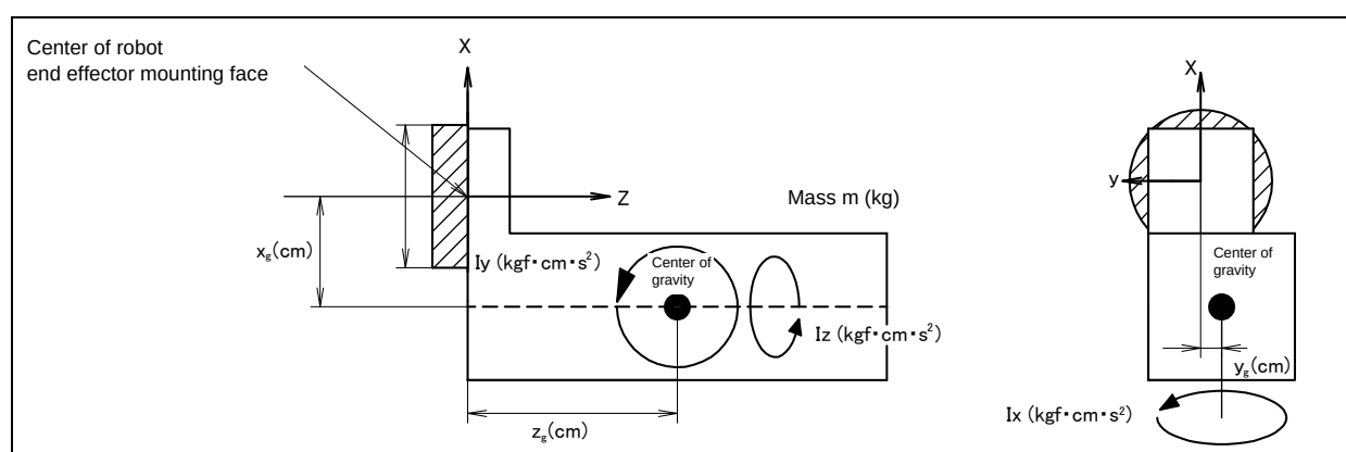
Fig. 4.2 (a) Standard tool coordinate
